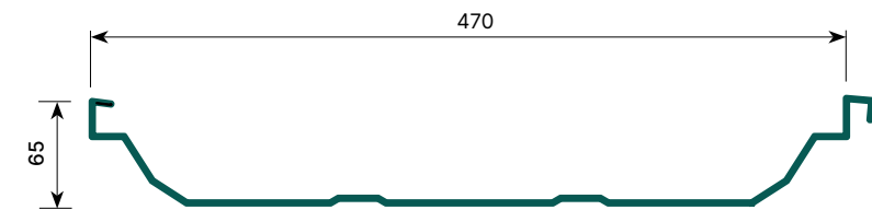
TÔN SÓNG SEAMLOCK | LOCKSEAM PANEL
