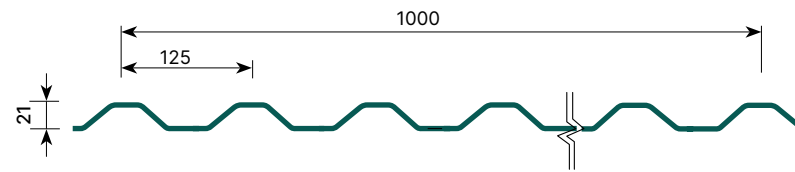
TÔN 9 SÓNG VUÔNG | 9 RIBS PROFILE PANEL
