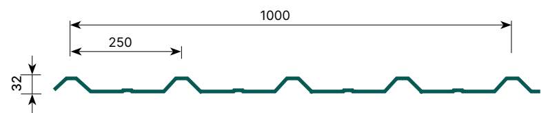
TÔN 5 SÓNG | 5 RIBS PROFILE PANEL
