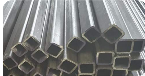
HỘP 40*40*3MM L0.96M/L1.8/L2.4M/L3M/L4.8M MẠ KẼM BOX 40*40*3MM L0.96M/L1.8/L2.4M/L3M/L4.8M ZINC PLATED
